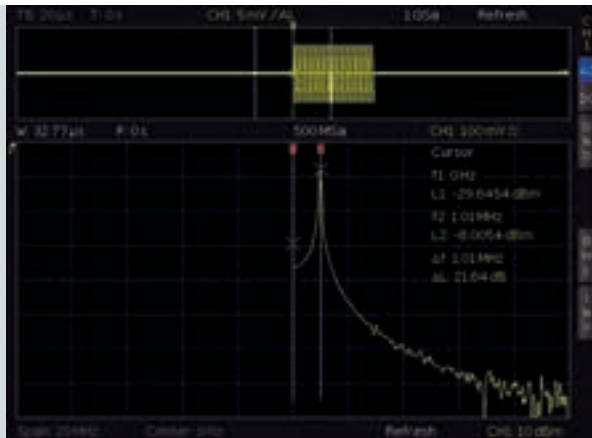
Figure 4: Rectangular measurement window
